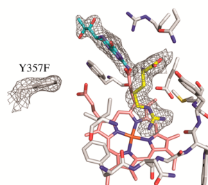
Figure 5. (A) Active site view of L-Arg and tetrahydrofolate bound to bsNOS (redrawn from PDB 1M7V). (B) Y357F bsNOS with L-Arg and H 4 B bound and shown with a 2F_o - F_c map contoured at 1.0\sigma . Protein residues of the NOS active site are white, heme is salmon, the pterin group is cyan, and L-Arg is yellow.
