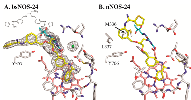
Figure 7. (A) Binding mode of 24 to bsNOS is extended to accommodate binding on the surface of the protein outside of the active site. The 2F_o - F_c map of 24 , H 4 B, and the active site chloride anion are contoured at 1.0\sigma . (B) 24 binding to nNOS results from the partially blocked active site, contributed by residues L337 and M336 (redrawn from PDB 4UPN). The color scheme shown has H 4 B in cyan, 24 in yellow, heme in salmon, and protein residues in white.
