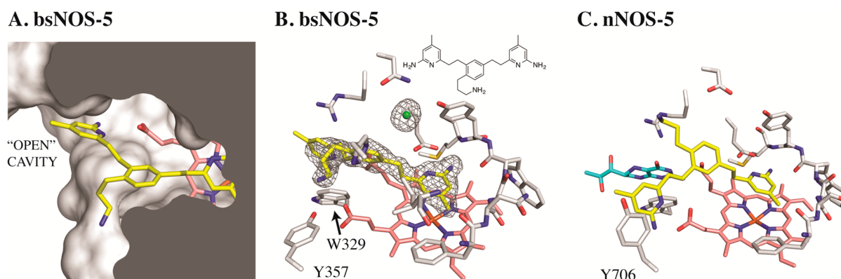
Figure 2. (A) 5 bound to bsNOS with the aminopyridine group bound to the heme propionate and exposed to a solvent-accessible surface that is unique to bNOS. (B) Stick representation and 2F_o - F_c at 1.0\sigma of 5 bound to bsNOS. (C) Stick representation of nNOS-5 (PDB 4IMT). In all representations, the heme group is salmon, 5 is yellow, a chlorine ion is green, H 4 B is cyan, and the protein residues are white.
