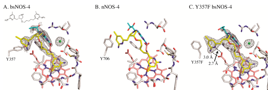
Figure 6. Inhibitor 4 bound to NOS active site shown as yellow sticks with the heme group in salmon, protein residues in white, and H 4 B in cyan. (A) The 2F_o - F_c map is contoured at 1.0\sigma for bsNOS-4. (B) 4 binds to nNOS by coordinating to the heme propionate group. (C) 4 binding to bsNOS is able to coordinate to the heme propionate only by introduction of mutation Y357F. The 2F_o - F_c map of 4 and H 4 B is contoured at 1.0\sigma .
