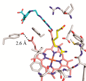
Figure 5. (A) Active site view of L-Arg and tetrahydrofolate bound to bsNOS (redrawn from PDB 1M7V). (B) Y357F bsNOS with L-Arg and H 4 B bound and shown with a 2F_o - F_c map contoured at 1.0\sigma . Protein residues of the NOS active site are white, heme is salmon, the pterin group is cyan, and L-Arg is yellow.
