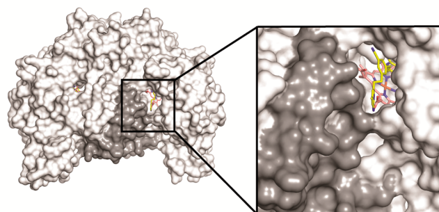
Figure 4. Inhibitor 3 induces a conformational change in both (A) bsNOS Y357 and (B) nNOS Y706. Rotation of Y357 in bsNOS opens access to a novel binding surface depicted in A. Surface representations of NOS oxygenase domains as dimers are white, with the N-terminal \text{Zn}^{2+} motif in gray. Heme groups are salmon, and ligands are yellow. The 2F_o - F_c map for bsNOS-3 is shown at 1.0\sigma . The nNOS-3 models were generated using PDB 4IMW.
