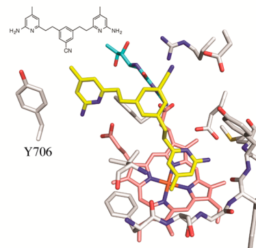
Figure 4. Inhibitor 3 induces a conformational change in both (A) bsNOS Y357 and (B) nNOS Y706. Rotation of Y357 in bsNOS opens access to a novel binding surface depicted in A. Surface representations of NOS oxygenase domains as dimers are white, with the N-terminal \text{Zn}^{2+} motif in gray. Heme groups are salmon, and ligands are yellow. The 2F_o - F_c map for bsNOS-3 is shown at 1.0\sigma . The nNOS-3 models were generated using PDB 4IMW.
